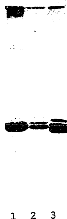
Fig. 2. Glycosylation pattern of PrA-Ala 294 . The yeast strains YS18 ( PRA1 ), SR1 ( pralΔEN::HIS3, pDP83pral-Ala 294 ) and SR2 ( pralΔEN::HIS3, pDP83PRA1 ) were preincubated for 20 min at 30°C with 60 μg/ml tunicamycin prior to labeling with [ 35 S]methionine for 30 min. Extract mixtures containing 100 μCi of radioactivity were applied on each lane. Immunoprecipitation was done using anti-PrA-serum; SDS-PAGE (12% gel): (Lane 1) SR2; (lane 2) YS18; (lane 3) SR1.
